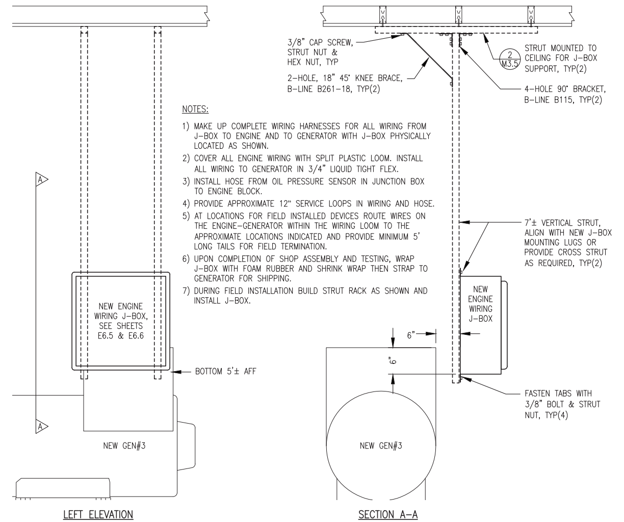
2 NEW ENGINE J-BOX INSTALLATION E3.5 NO SCALE
